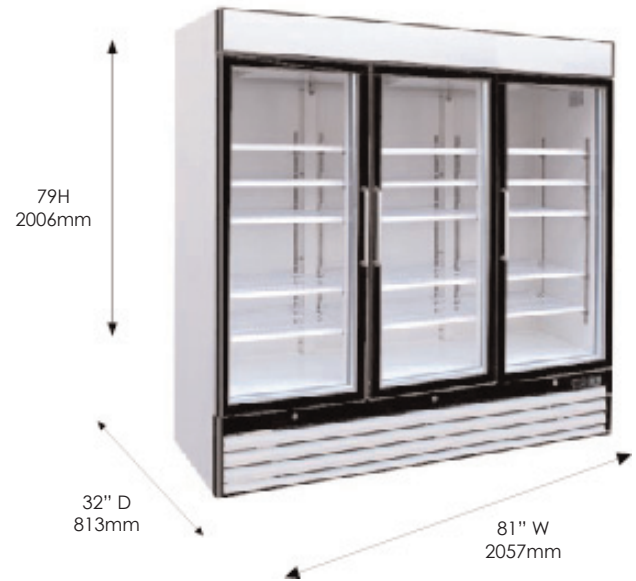
Model MXM3-72R
