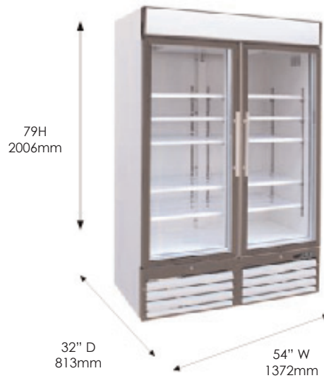
Model MXM2-48R
